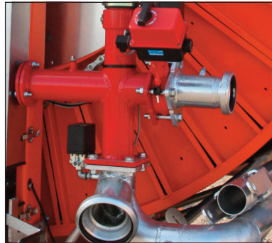
Discharge valve VD
