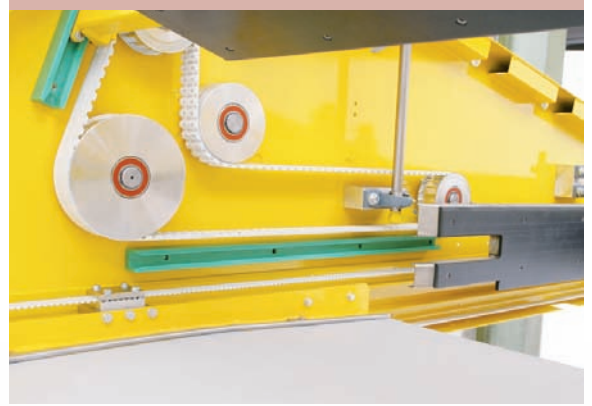
Toothed belt driven layer cross pusher
