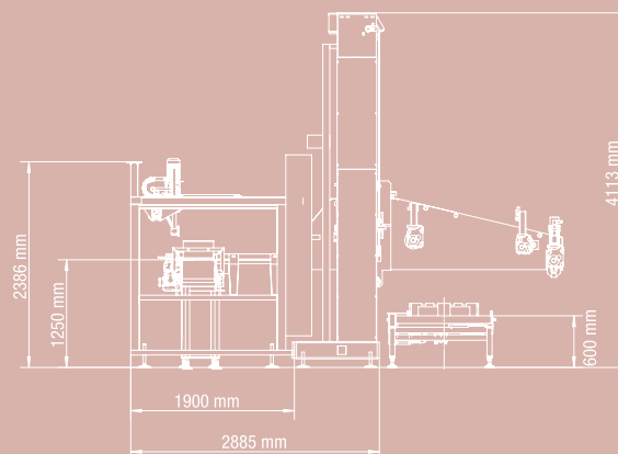
Side view of the machine type PK 110
