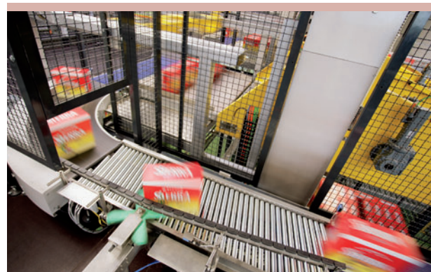
Case turning station at the infeed of the PK 110
