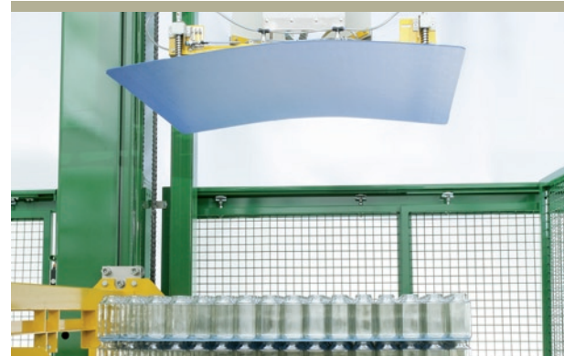
Intermediate layer remover on the DL 71
