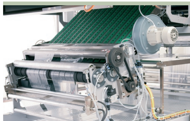
Film cutting unit for the double-laned product infeed of the SW 90 TM-60
