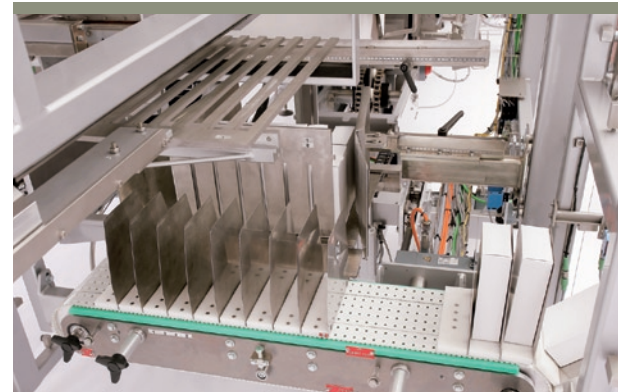
Paddle chain infeed of the VP 453
