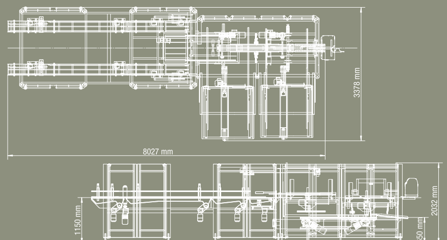
Top view of the machine type VP 453 Side view of the machine type VP 453
